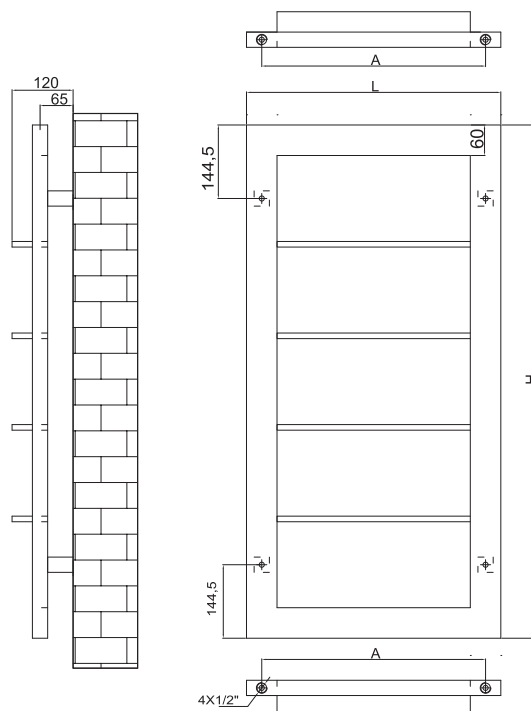
Hydraulic connections/Conexiuni hidraulice*
