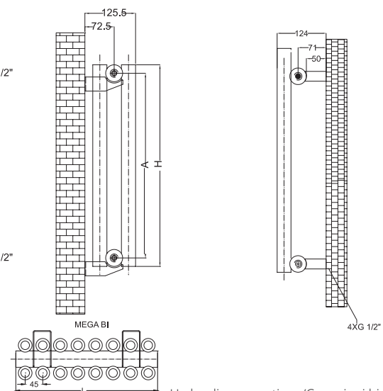
Hydraulic connections/Conexiuni hidraulice*
