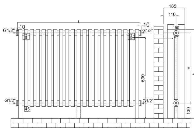
Hydraulic connections/Conexiuni hidraulice*
