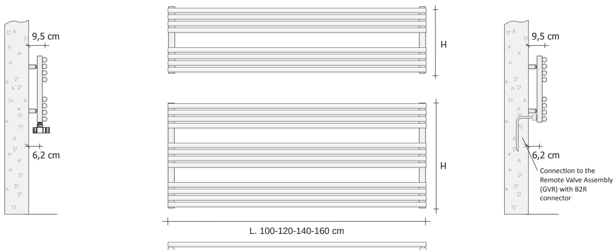
STANDARD HYDRAULIC VERSION (Connectors OB1)
